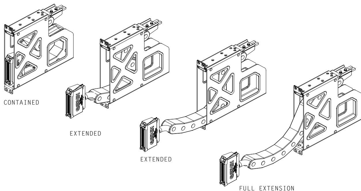
Figure 2-1. CHiPS Harness
